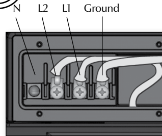
240 VAC Heater (4KW or 2 KW)
