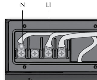
120 VAC Heater (1 KW)
